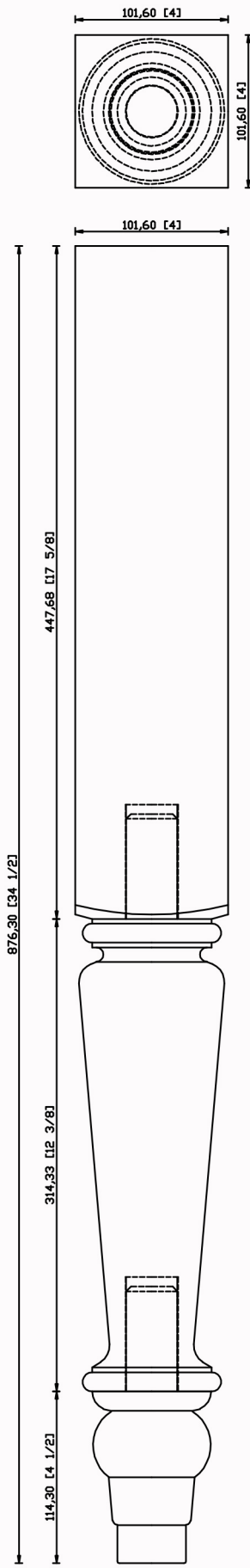
SY-L-5054 4" x 4" x 34-1/2"
