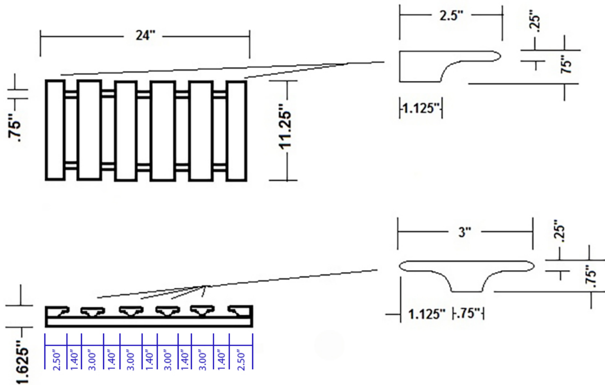
24" STEMWARE RACK
