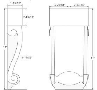
CA123 (corner corbel)
