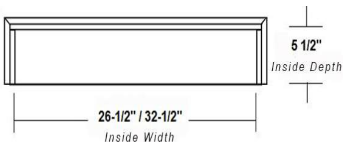
Reeded Molding Detail
