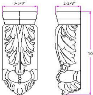
CA122 (corner corbel)
