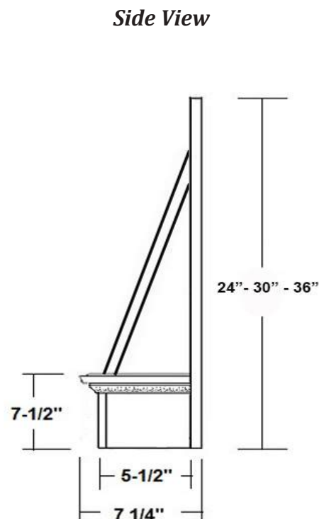
Acanthus Molding Detail
