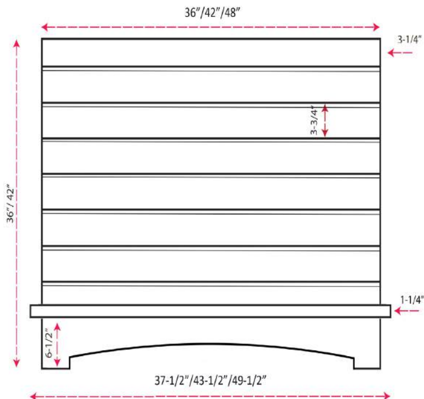
Front View
